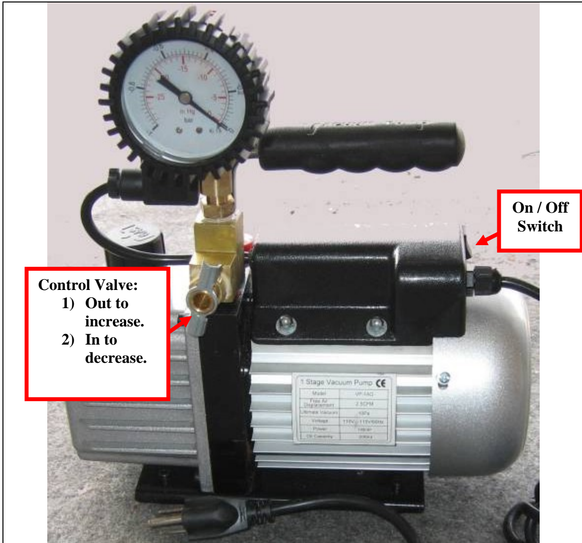
2CFM Vacuum Pump with Gage
